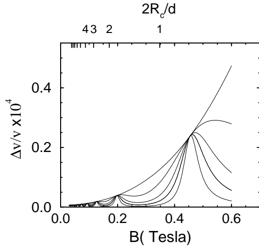
FIG. 2. Velocity shift \Delta v/v of SAW as a function of the magnetic field. The values of all the parameters are the same as in Fig.1.
